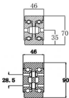
Installation Diagram
