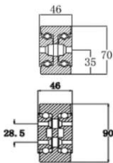
Installation Diagram
