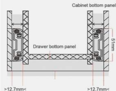
Installation dimensions
